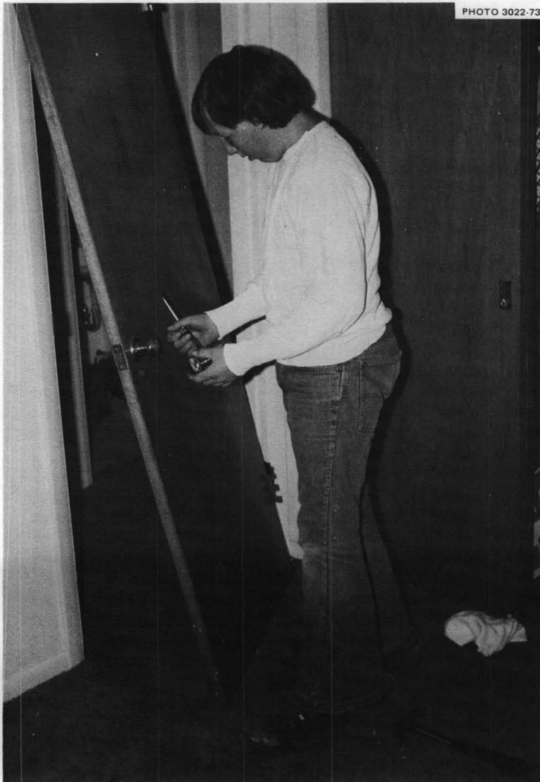
Fig. 2.1. Start by an untrained, unskilled family of the second proof-testing of the written instructions for building a Door-Covered Trench Shelter. Starting at 6 AM on November 24, 1973, son Tad, age 14, and other children removed the doorknobs from one of the six interior doors that this fatherless family of six readied for use.
